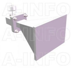
LB-90-15-C-7SPO Standard Gain Horn Antenna 8.2-12.4GHz 15dB Gain 7mm
