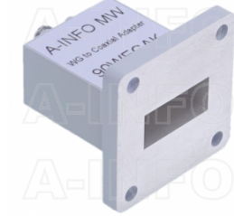
90WECAK Endlaunch Rectangular Waveguide to Coaxial Adapter 8.2-12.4GHz WR90 to 2.92mm Female
