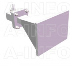
LB-90-15-C-TFSP Standard Gain Horn Antenna 8.2-12.4GHz 15dB Gain TNC Female
