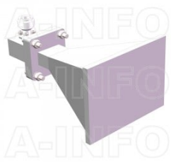
LB-90-15-C-NFSP Standard Gain Horn Antenna 8.2-12.4GHz 15dB Gain N Type Female
